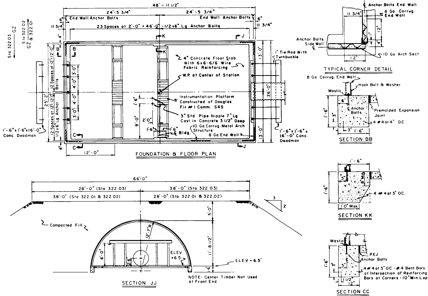
Fig. 3—Plan and details of typical 25-ft-span test structure.
